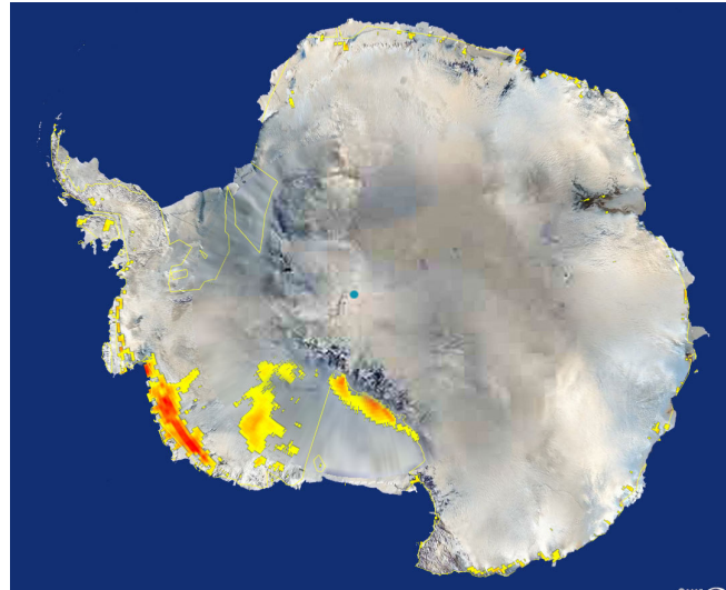
NASA's QuikScat satellite detected extensive areas of snowmelt, shown in yellow and red, in west Antarctica in January 2005. Image credit: NASA/JPL
